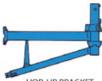
HOP-UP BRACKET 2 BOARD 565MM 3 BOARD 795MM
